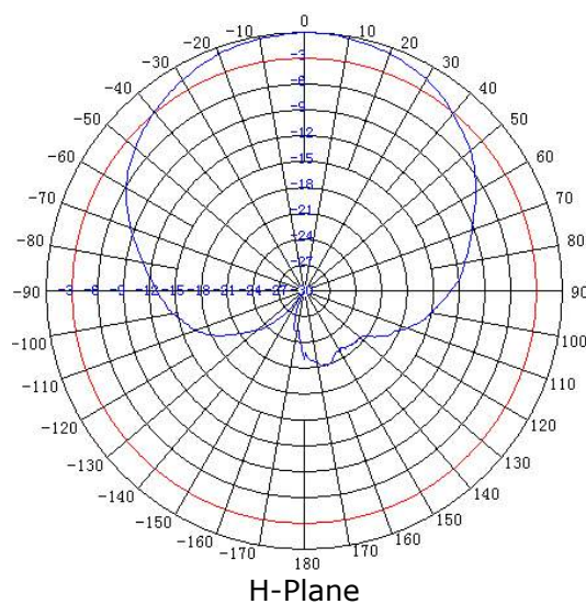
Radiation Pattern: CA-P2004
